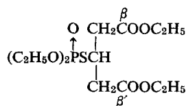
\beta -Glutarate malaoxon
